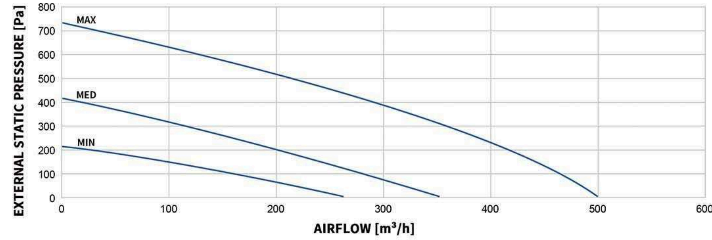
MODEL: WESTON-EV-CT-CORE-500
