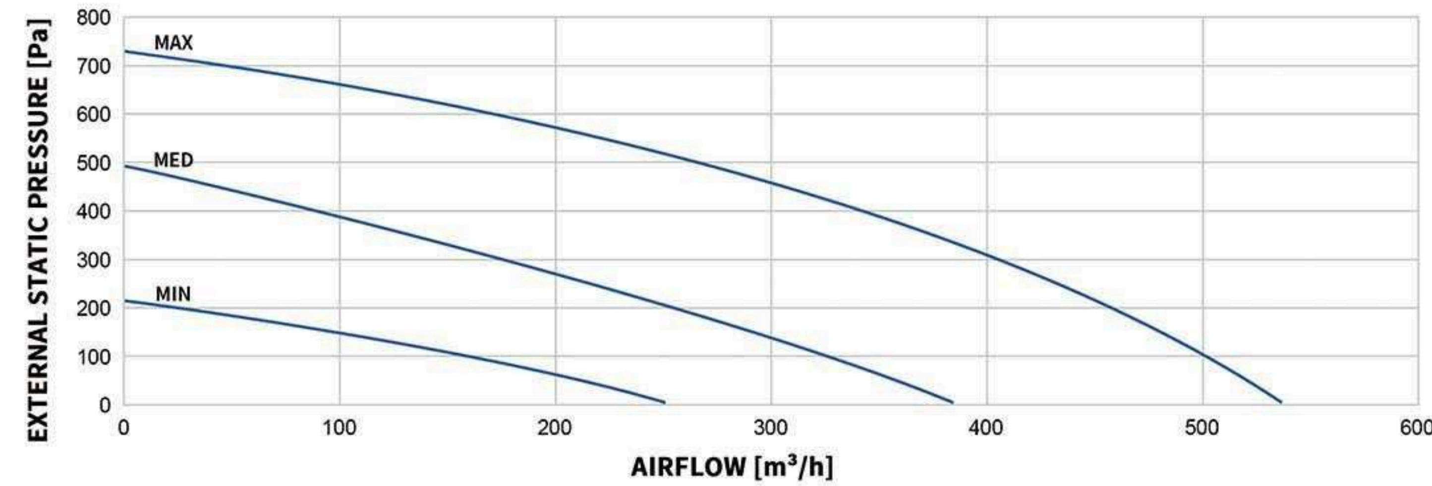
MODEL: WESTON-EV-CT-CORE-550
