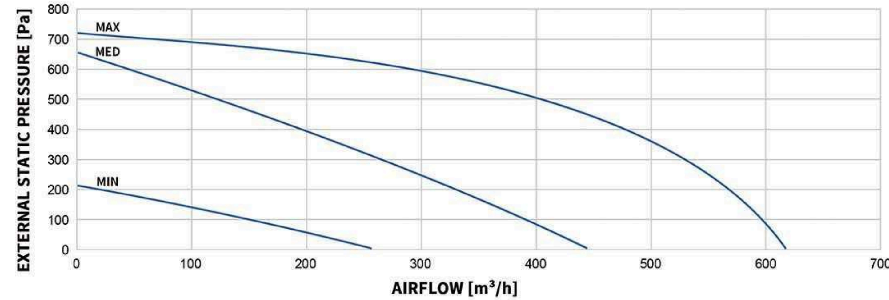
MODEL: WESTON-EV-CT-CORE-600
