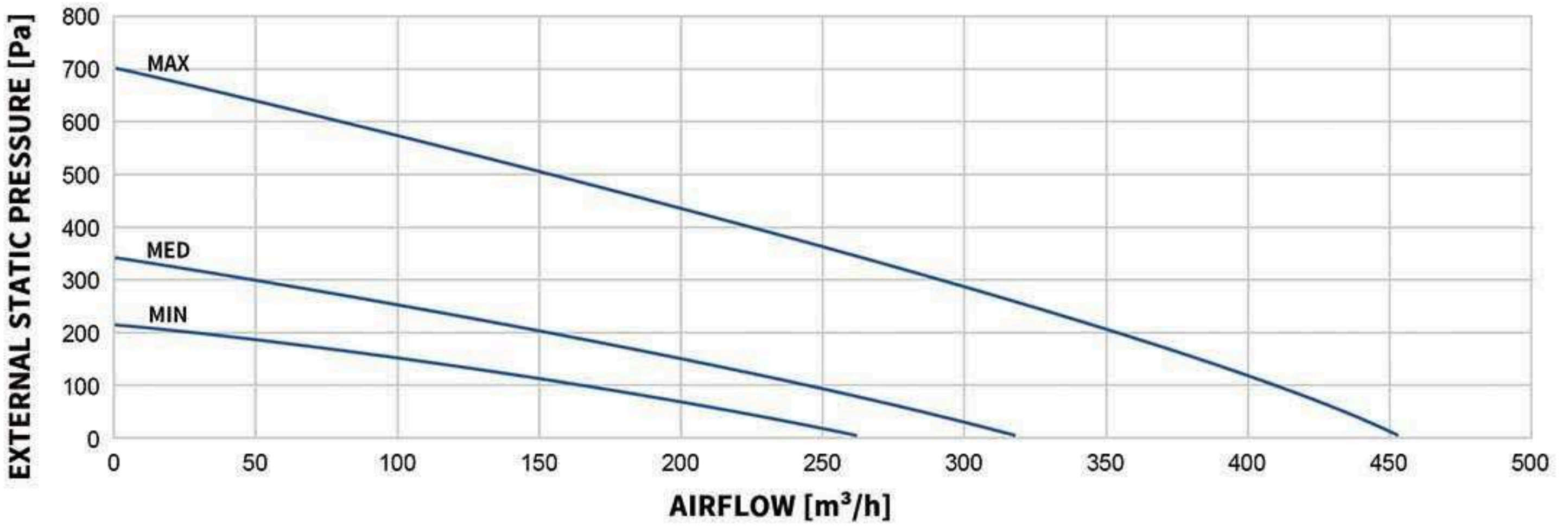
MODEL: WESTON-EV-CT-CORE-450
