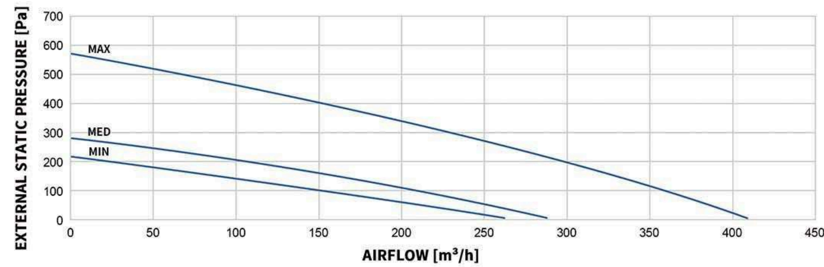
MODEL: WESTON-EV-CT-CORE-400
