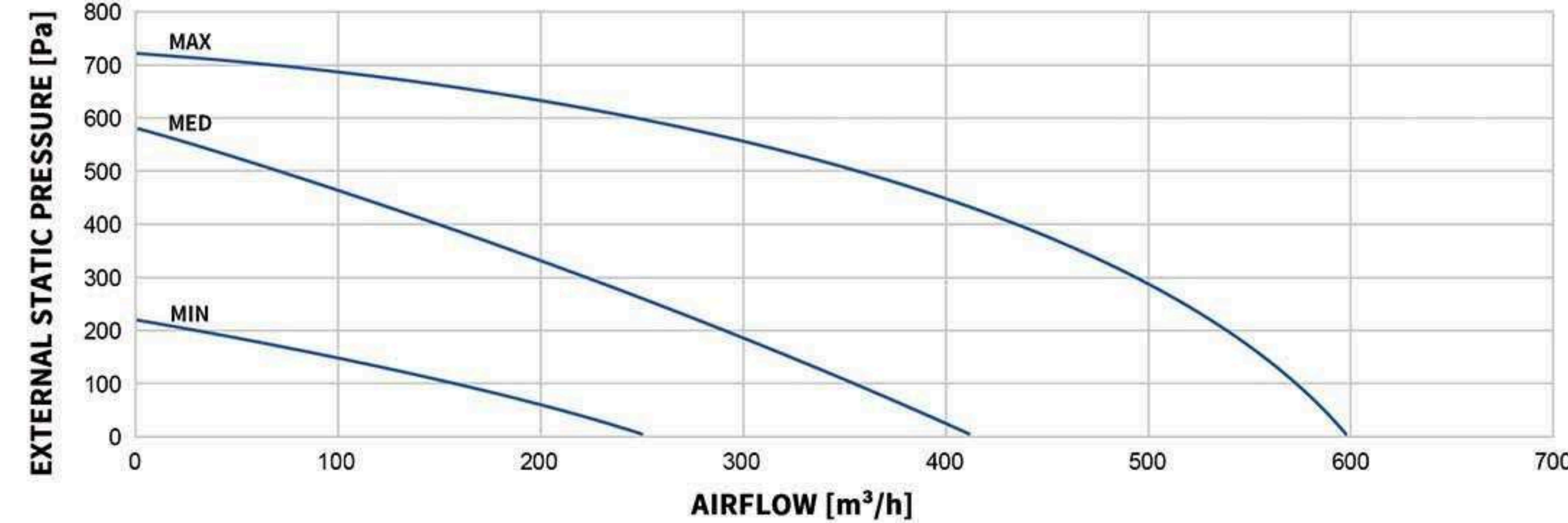
MODEL: WESTON-EV-CT-CORE-600
