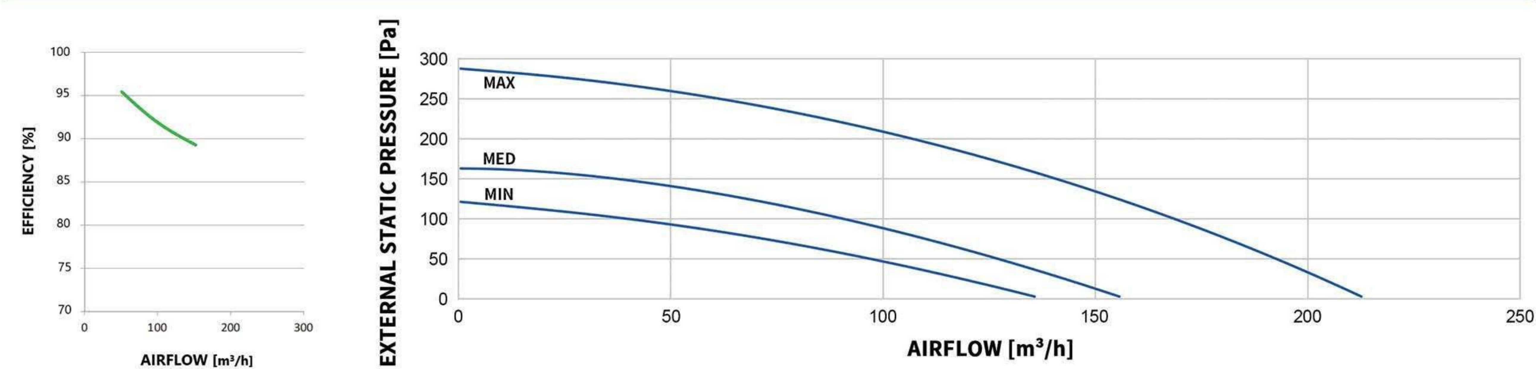
MODEL: W150-ERV-B-Z-EC
