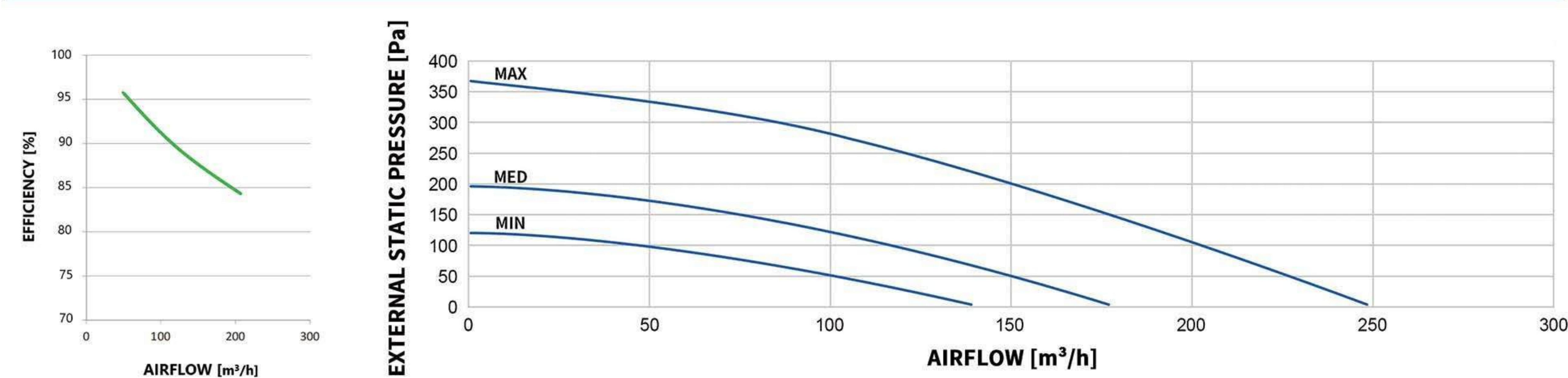
MODEL: W190-ERV-B-Z-EC
