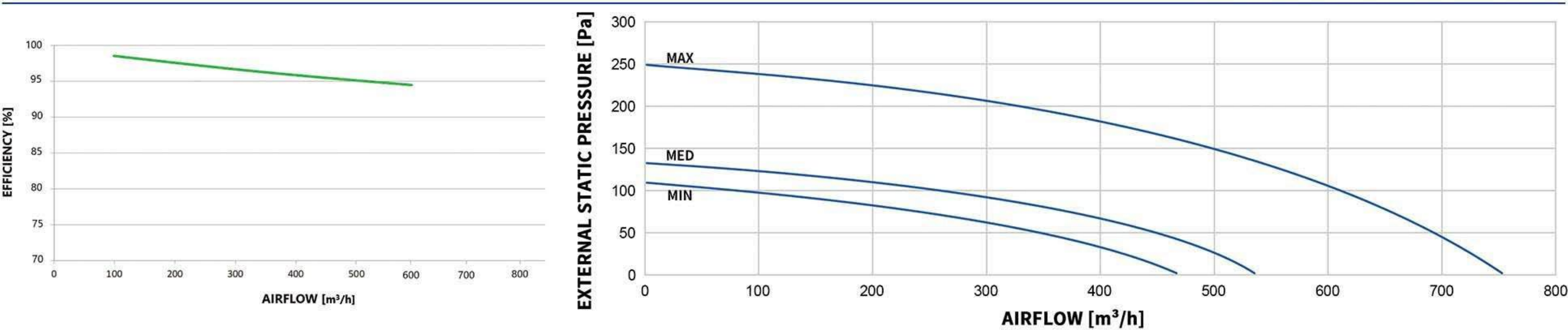
MODEL: W600-ERV-B-Z-EC
