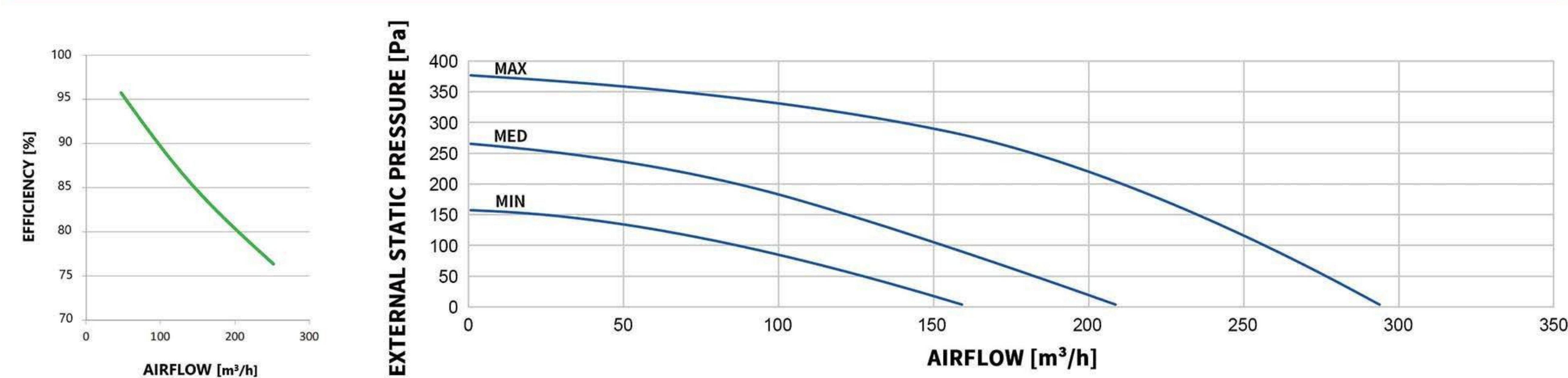
MODEL: W240-ERV-B-Z-EC
