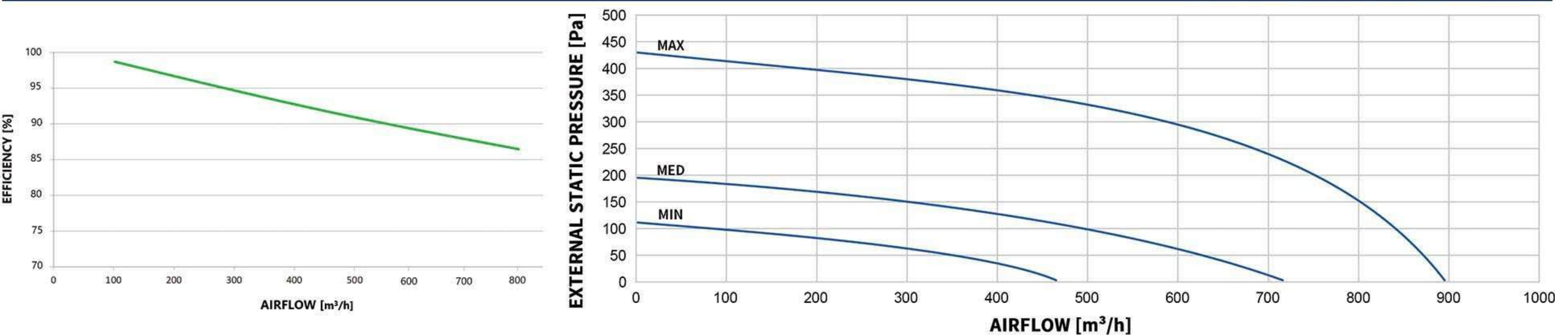
MODEL: W800-ERV-B-Z-EC
