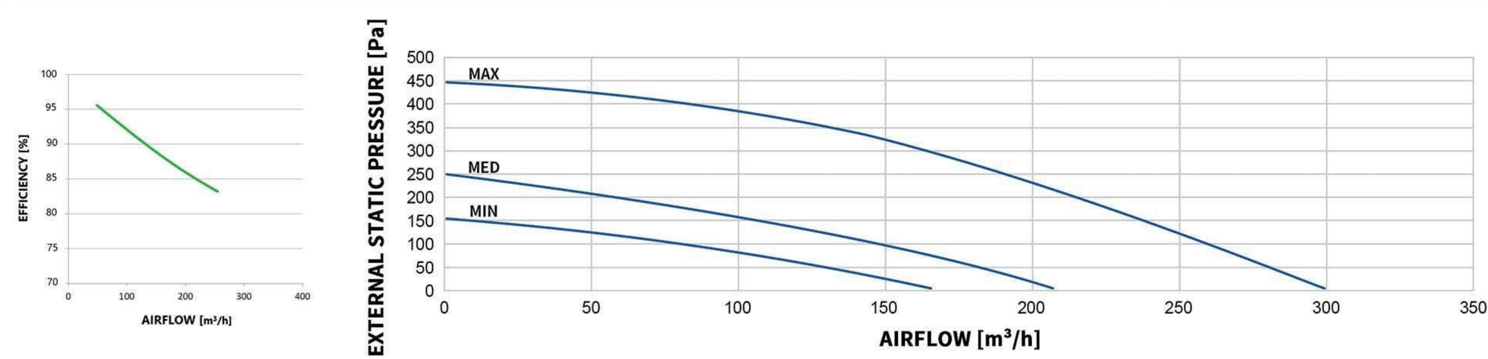
MODEL: W250-ERV-B-Z-EC
