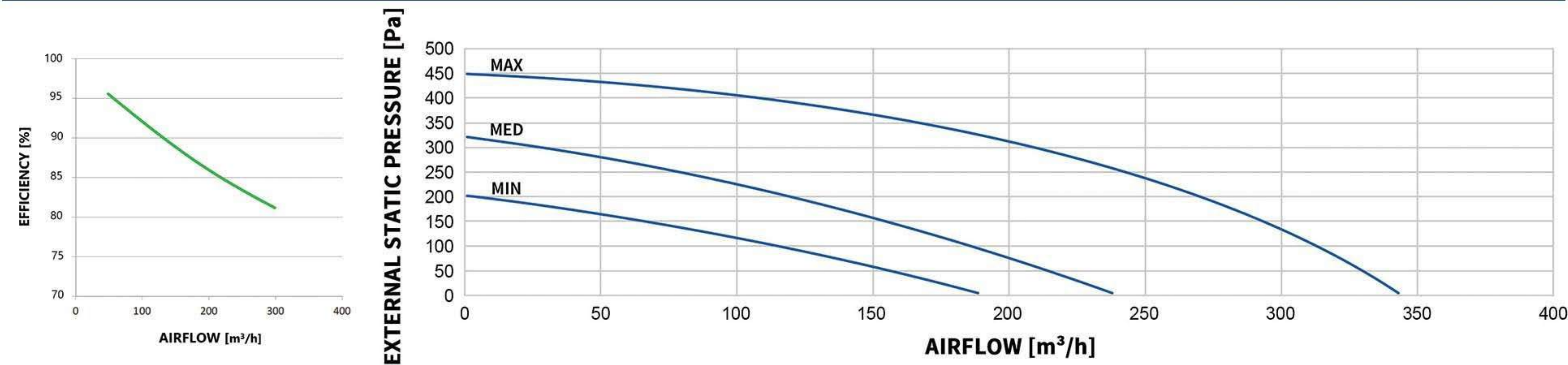
MODEL: W300-ERV-B-Z-EC
