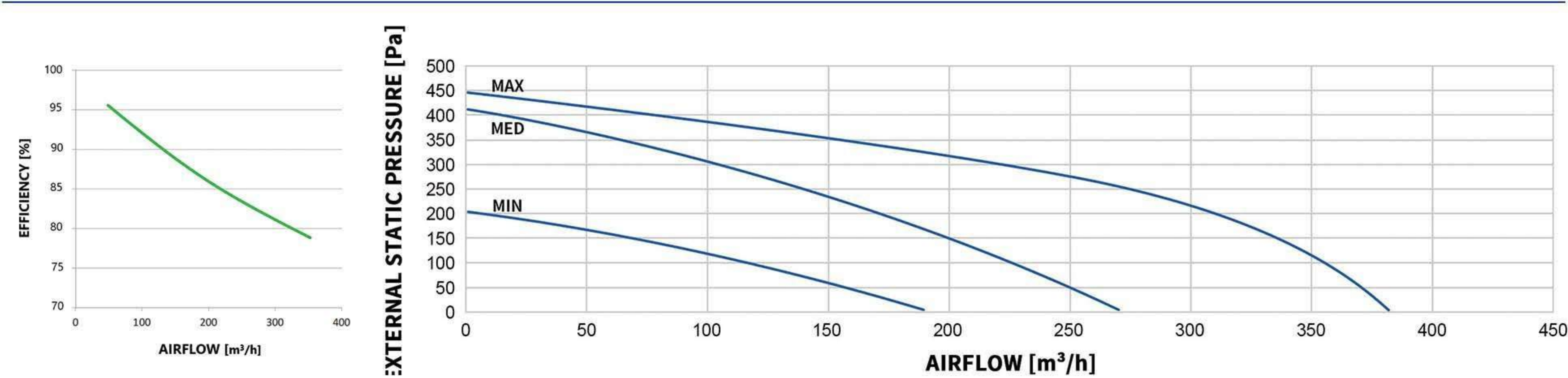
MODEL: W350-ERV-B-Z-EC
