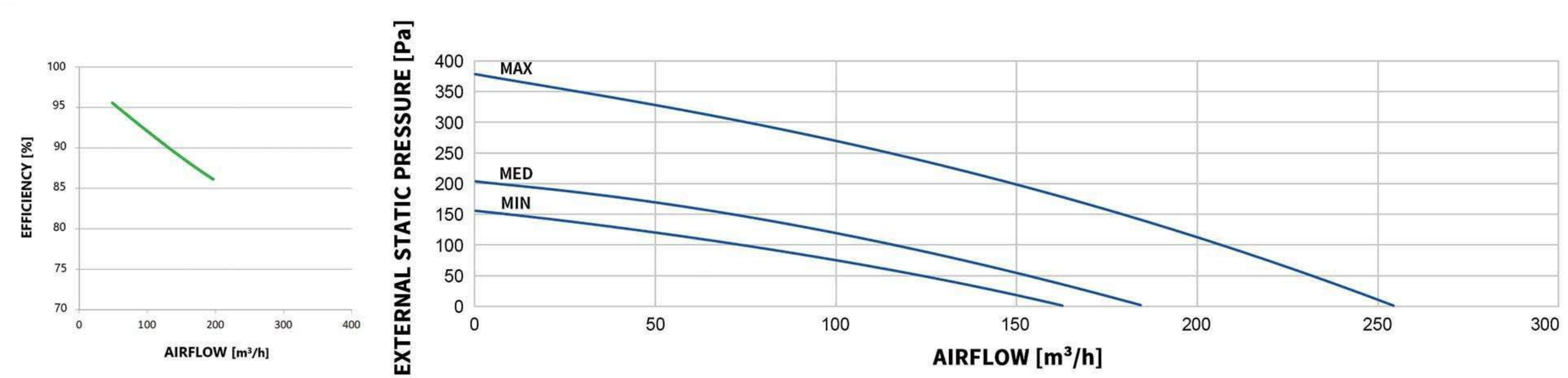
MODEL: W200-ERV-B-Z-EC
