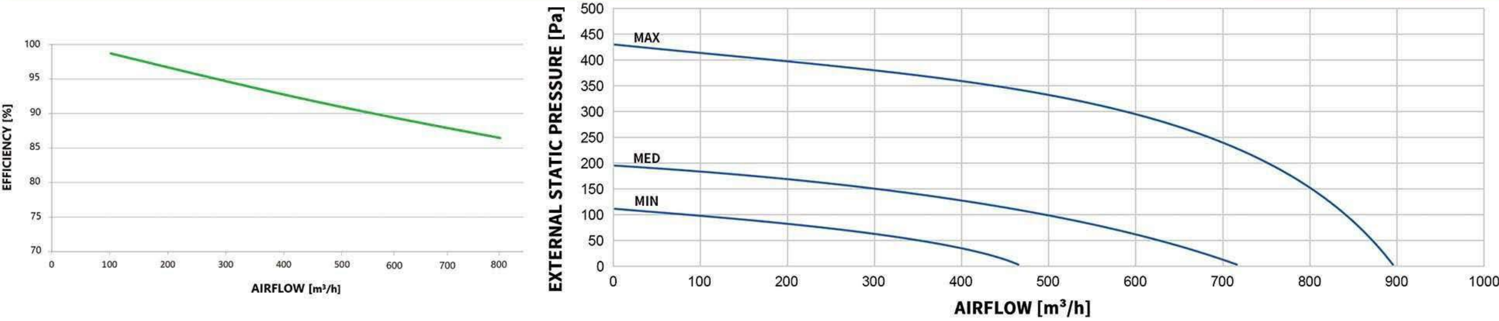
MODEL: WESTON-EV-CT-PRIME-800
