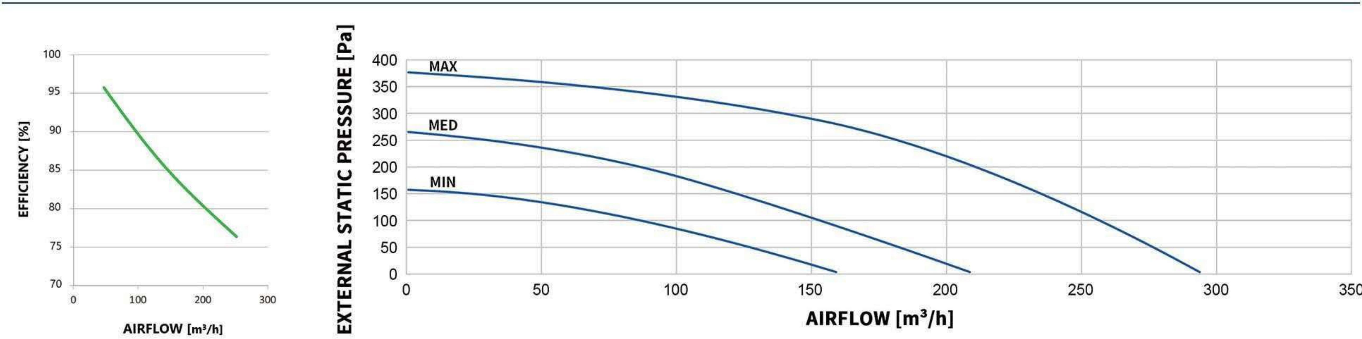
MODEL: WESTON-EV-CT-ESSE-240
