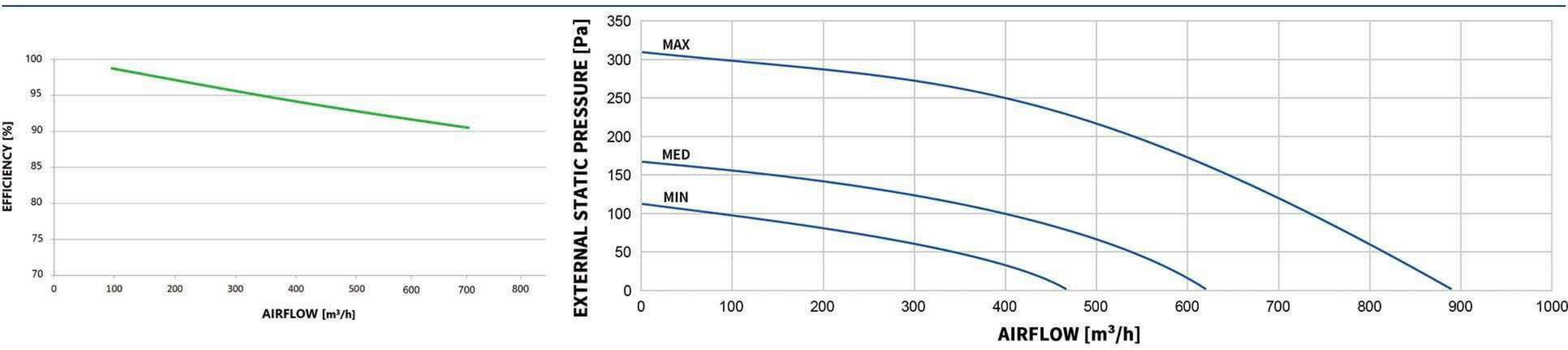
MODEL: WESTON-EV-CT-PRIME-800
