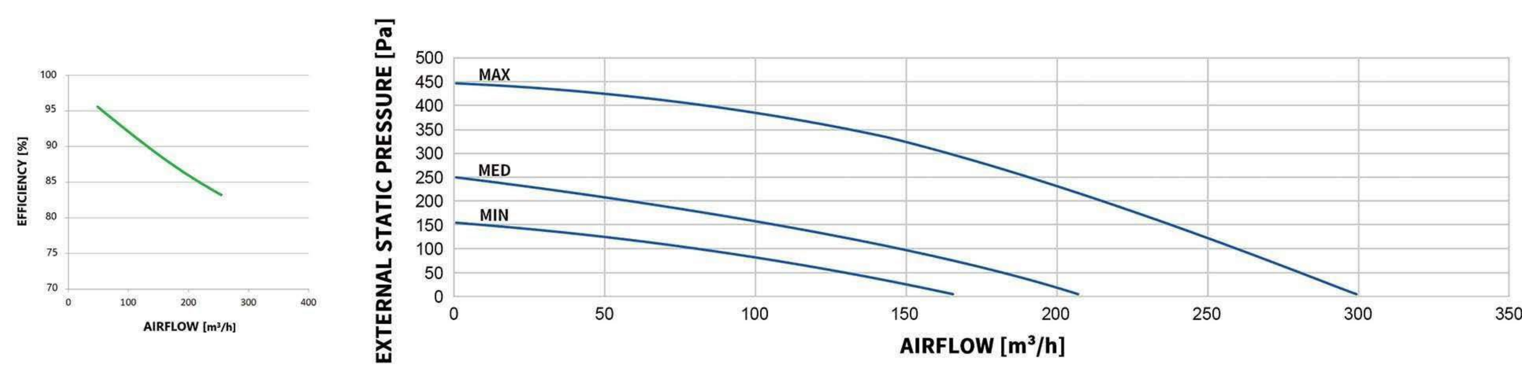
MODEL: WESTON-EV-CT-FLOW-250
