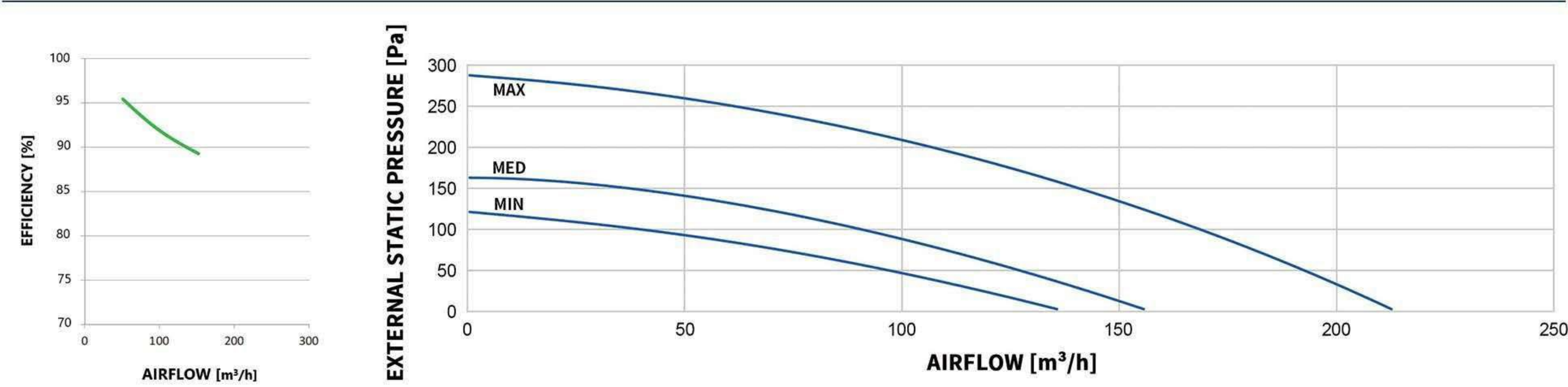
MODEL: WESTON-EV-CT-ESSE-190
