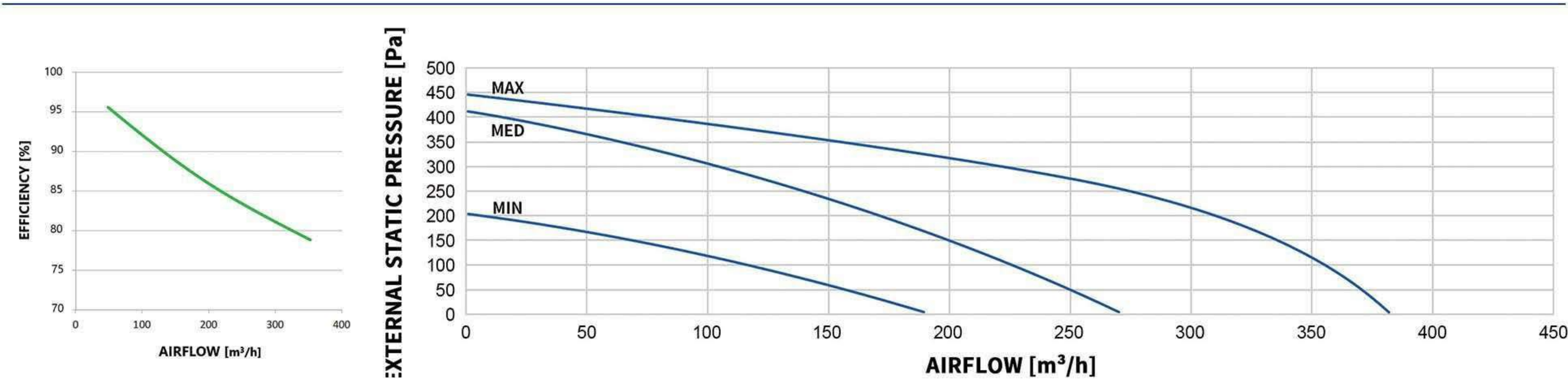
MODEL: WESTON-EV-CT-FLOW-350
