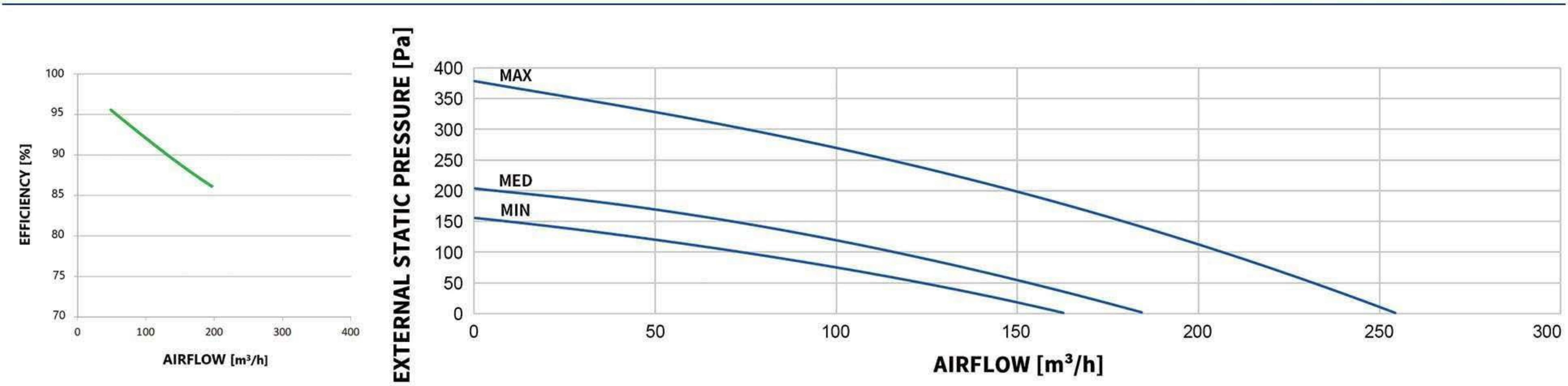
MODEL: WESTON-EV-CT-FLOW-200
