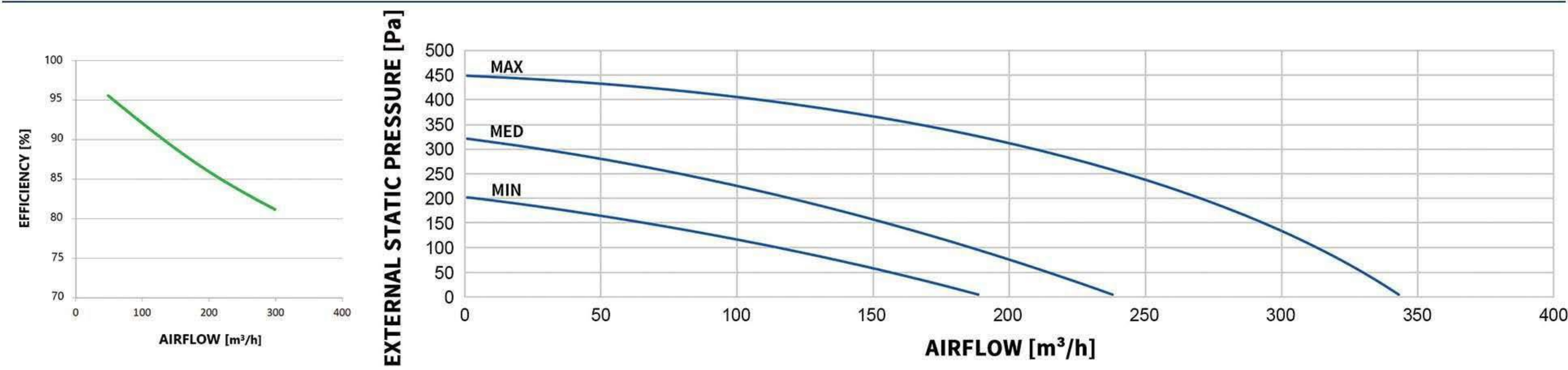
MODEL: WESTON-EV-CT-FLOW-350
